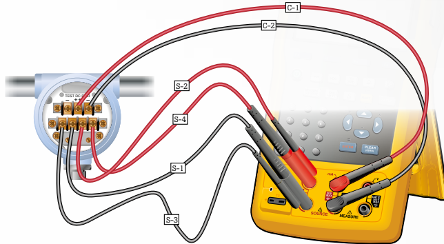
RTD transmitter calibration connection
