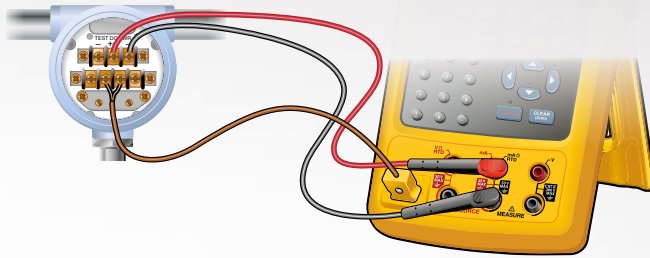
TC transmitter calibration connection
