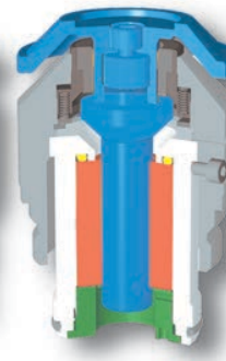
Negative free deformation, gas
