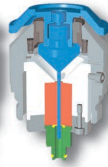
Simple free deformation, oil
